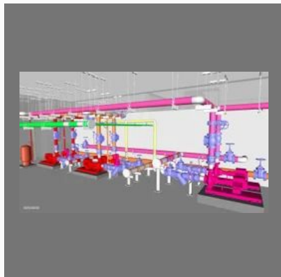
Fire Pump Room Design & Installation
